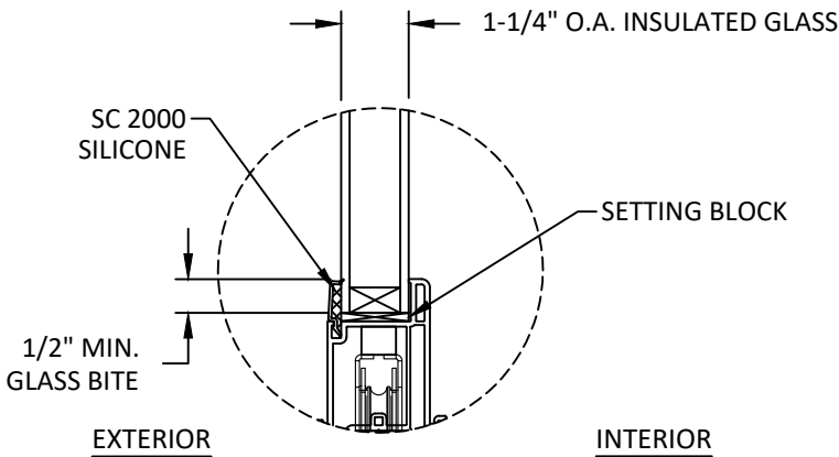
GLAZING DETAIL 1
